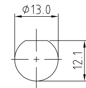
RECOMMENDED TNC MOUNTING HOLE
