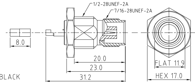
RP TNC DETAIL DRAWING
